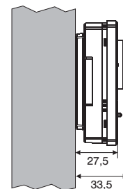
Remote probe
